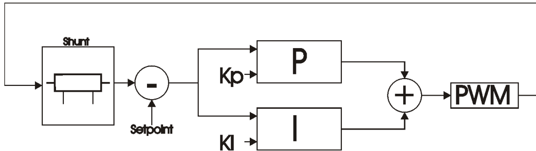
Simplified PI current regulator
