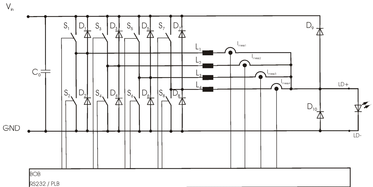
Operation principle of the LDP-CW 20-50 driver
