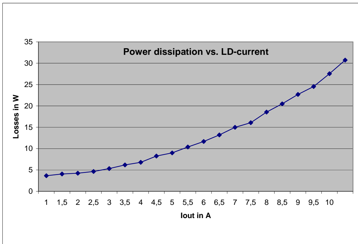
Power dissipation over output current
